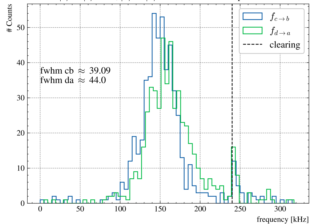
|c\rangle \rightarrow |b\rangle 18db, |d\rangle \rightarrow |a\rangle 12db microwave amplification
