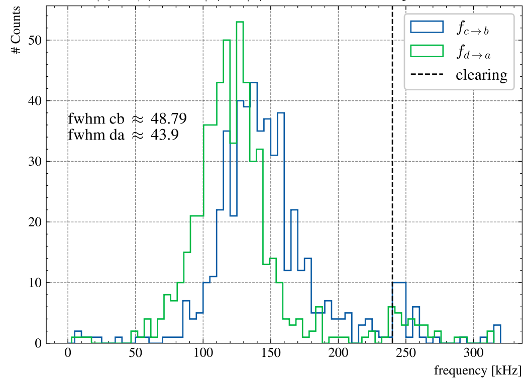
|c\rangle \rightarrow |b\rangle 18db, |d\rangle \rightarrow |a\rangle 12db microwave amplification
