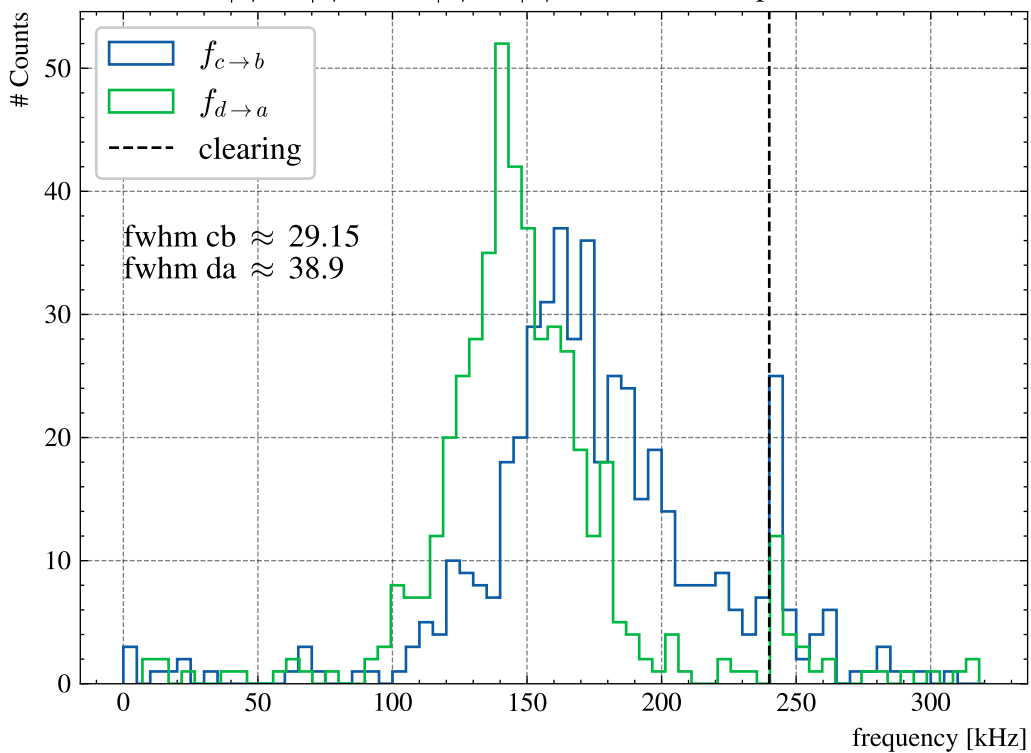
|c\rangle \rightarrow |b\rangle 18db; |d\rangle \rightarrow |a\rangle 18db microwave amplification
